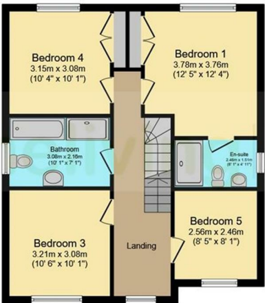
First Floor Floor area 63.1 sq.m. (679 sq.ft.)
